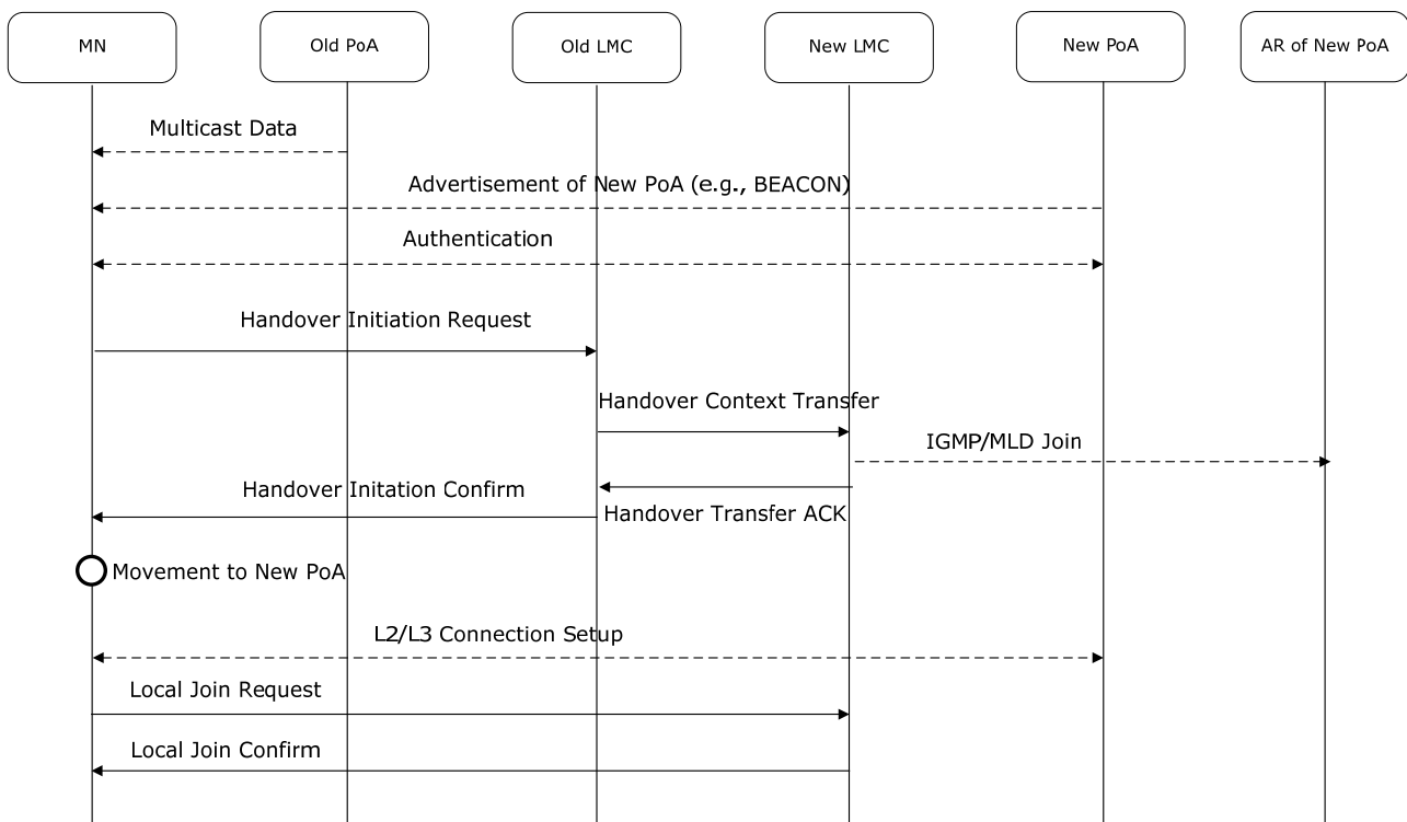
Figure 7 – Handover Support
